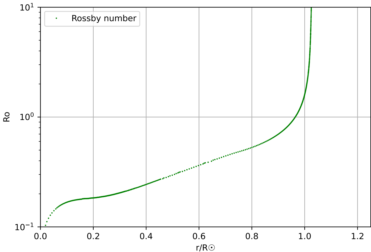
Rossby number, profile 151, age 5.58 \times 10^9
